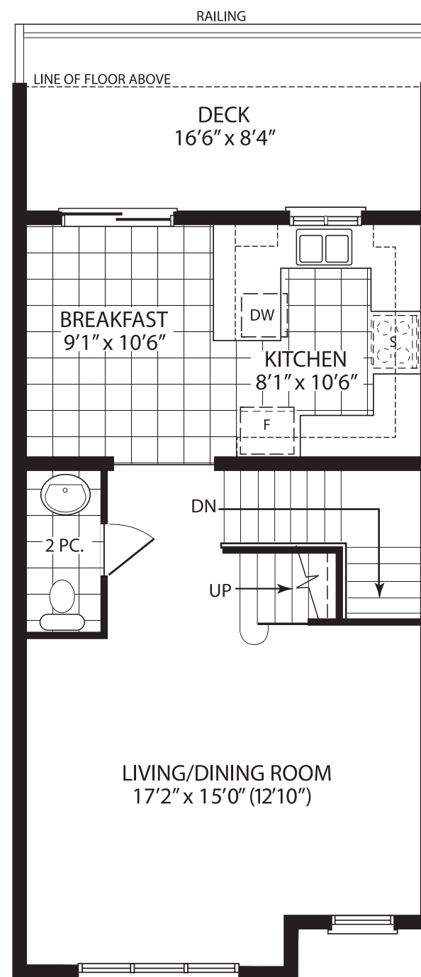
MAIN LEVEL ELEVATION B
