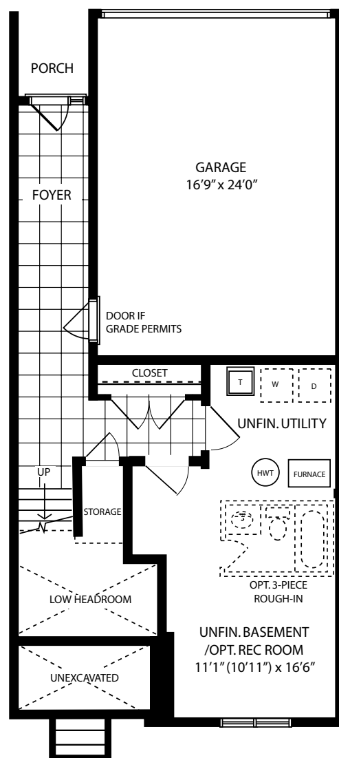
Lower Level Elev A
